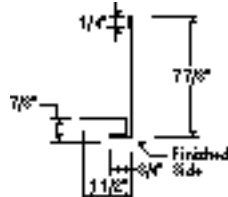
7 Overhead Door Trim
