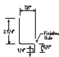
13 Double Angle
