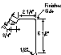
22 Eave & Gable Trim
